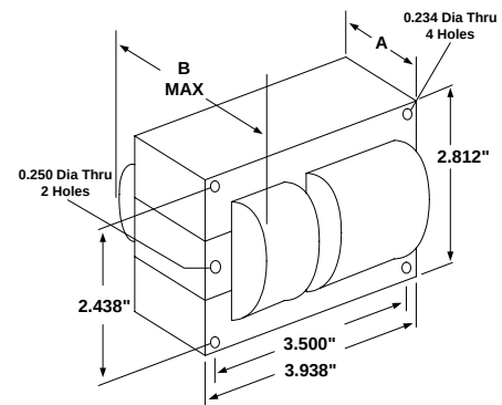
Reference Drawing
